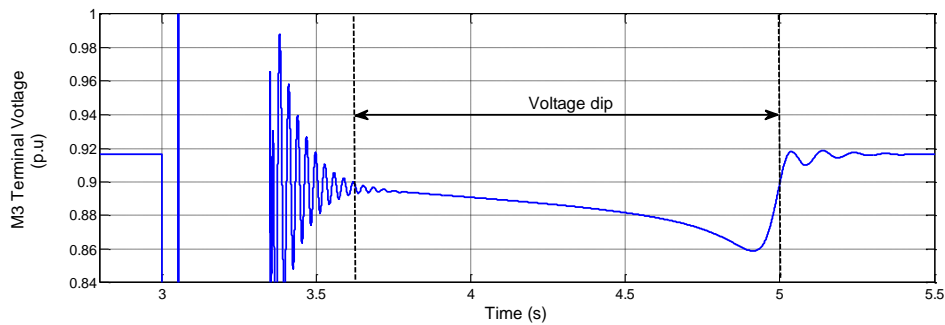
Figure 5.6: Voltage dip during M3 start-up following Flt-A using conventional reclosing.
