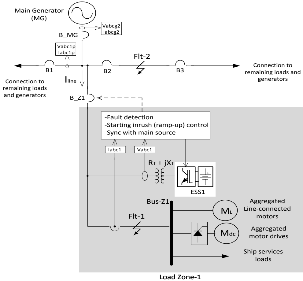
Figure 7.9: Test System with aggregated models of line-connected motors, ASDs and ship service loads
